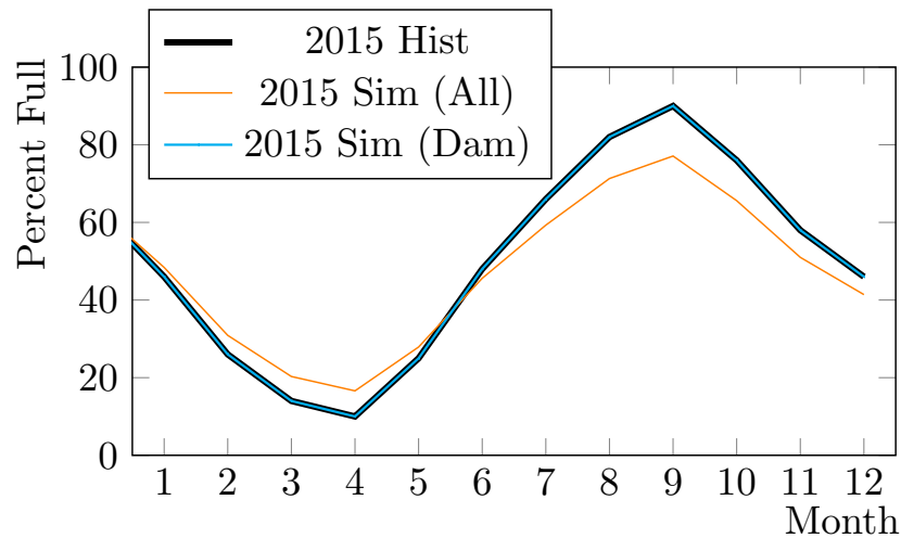
Figure 11: Swiss hydro storage level profile over the year (% full).
