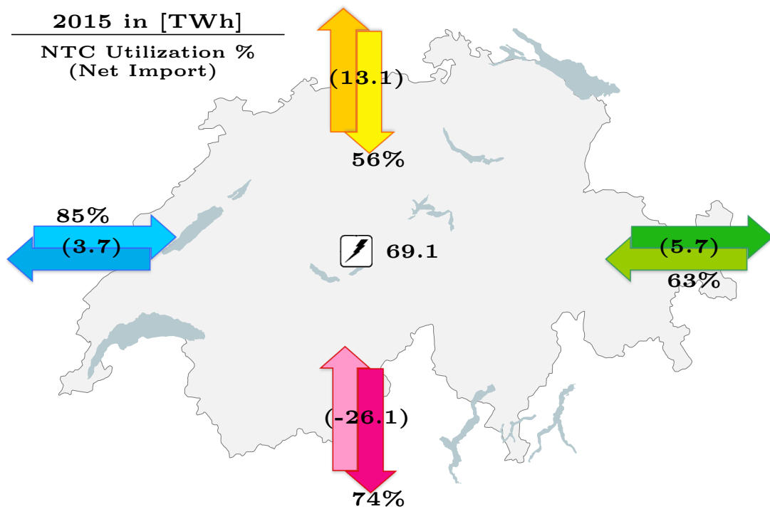
Figure 10: Annual average NTC utilization to each neighbor (net imports are in parenthesis).
