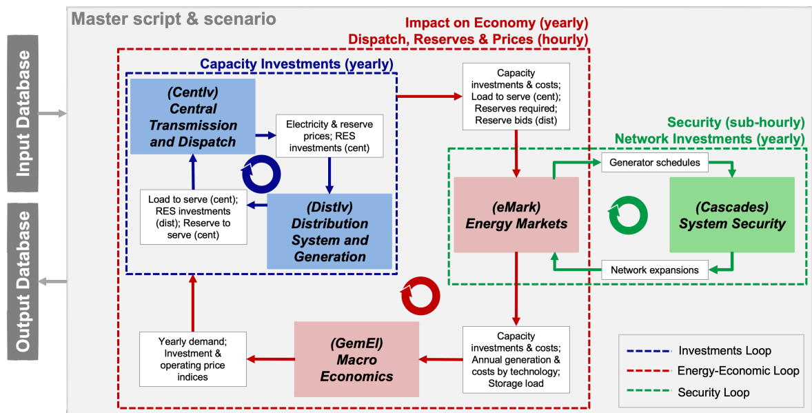
Figure 6: Illustration of the integration and interfacing of the various modules used in Nexus-e.
