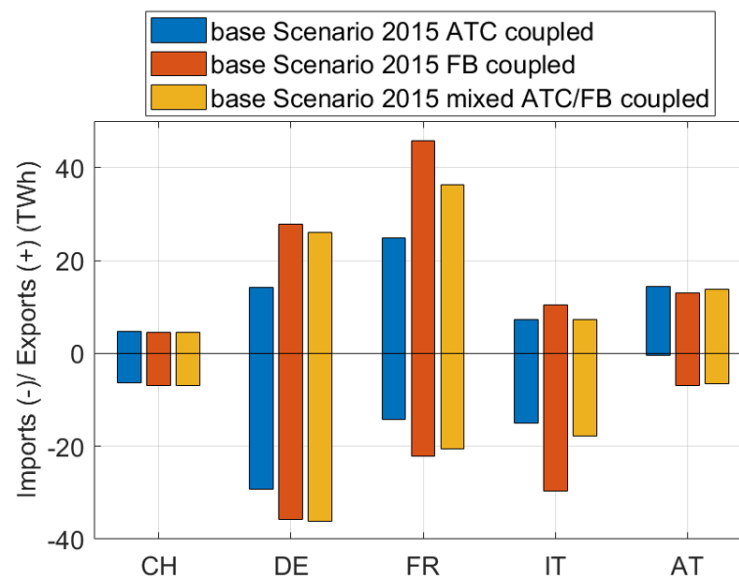
Figure 12: Transitioning from an ATC coupled market structure to a mixed or FB coupled structure can improve the utilization of transmission capacities.
