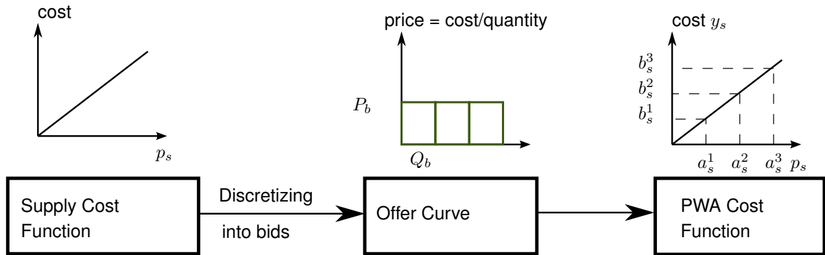
(a) Supply offer modeling. Any convex cost function is discretized into offers that are further processed into a PWA cost function. In this way, the MILP problem can be translated in a less complex LP clearing problem.
