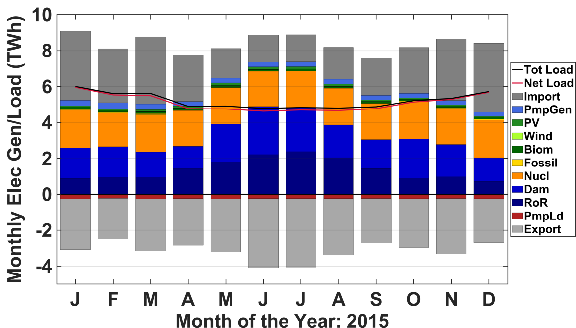
Figure 7: Monthly electricity supply/demand for Switzerland: production by technology type, imports, exports, total load, net load, and pump load.
