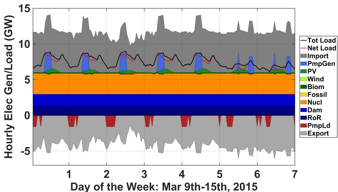
Figure 8: Hourly electricity supply/demand for Switzerland over a one week period (March 9th-15th): production by technology type, imports, exports, total load, net load, and pump load.
