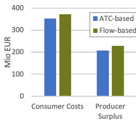
Figure 13: Annual Swiss consumer costs and producer surplus assuming an ATC or FB coupled market.
